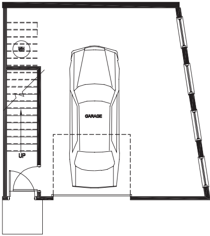
1st Floor
